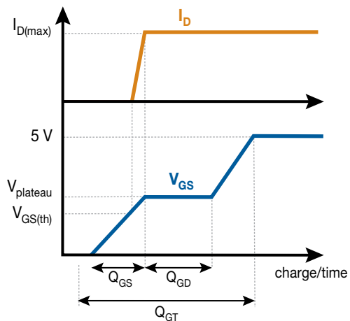
Figure 13. Typical Gate Charge Test Waveform
