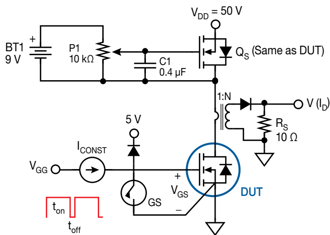
Figure 14. Charge Test Circuit
