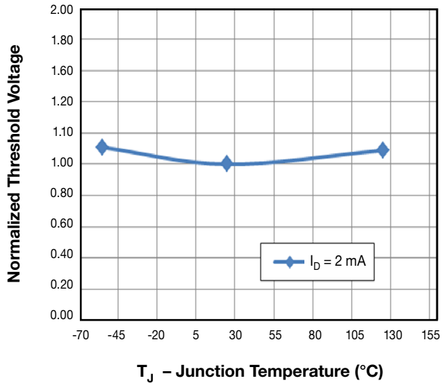
Figure 4. Normalized Threshold Voltage
