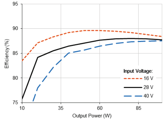
4.1.6 VHR100+2828S Efficiency (%) vs. Output Power (W)
